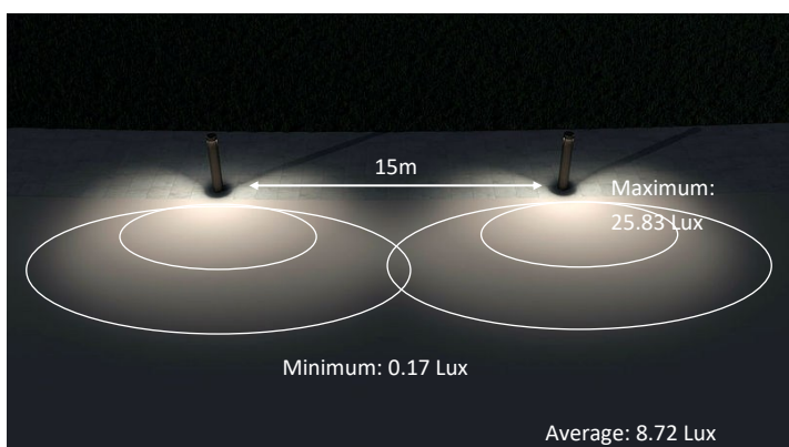
PP5: 15m spacing—Horizontal levels
