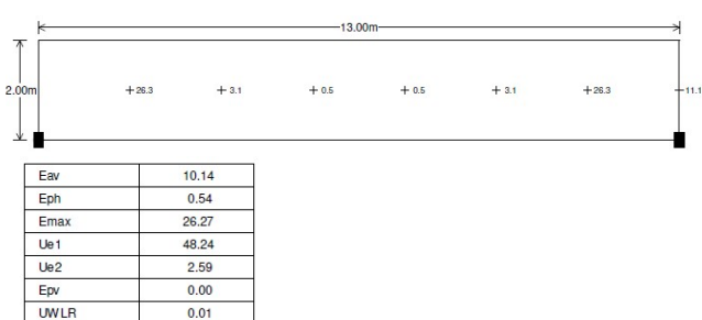
PP3: 13m spacing—Horizontal levels
