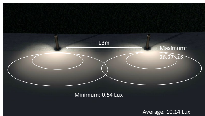
PP3: 13m spacing—Horizontal levels
