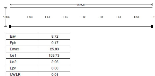
PP5: 15m spacing—Horizontal levels
