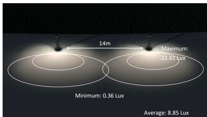
PP4: 14m spacing—Horizontal levels
