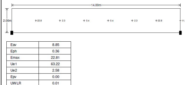
PP4: 14m spacing—Horizontal levels
